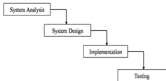
Fig. 1: Waterfall Model
